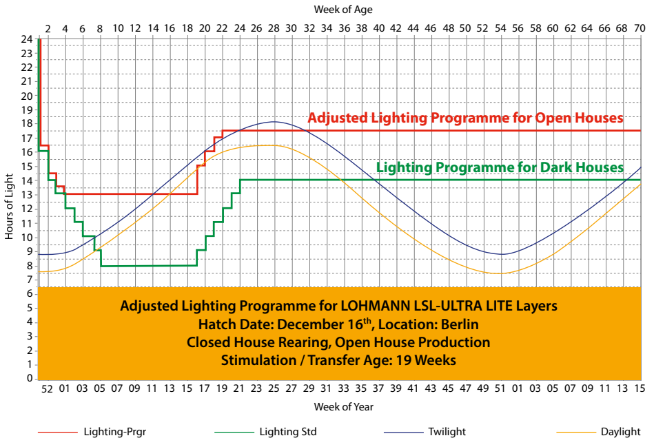
An example of a lighting programme for LOHMANN LSL-ULTRA LITE Layers adjusted to location, condition and requirements by LOHMANN lighting programme tool
